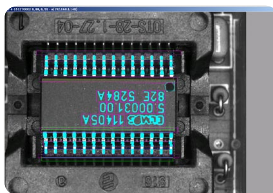
Image 1: Kontron's KISS servers are used by Asentics, for example, in a microchip inspection system for components that control car airbags. The picture shows the relevant inspection areas for the chip.
